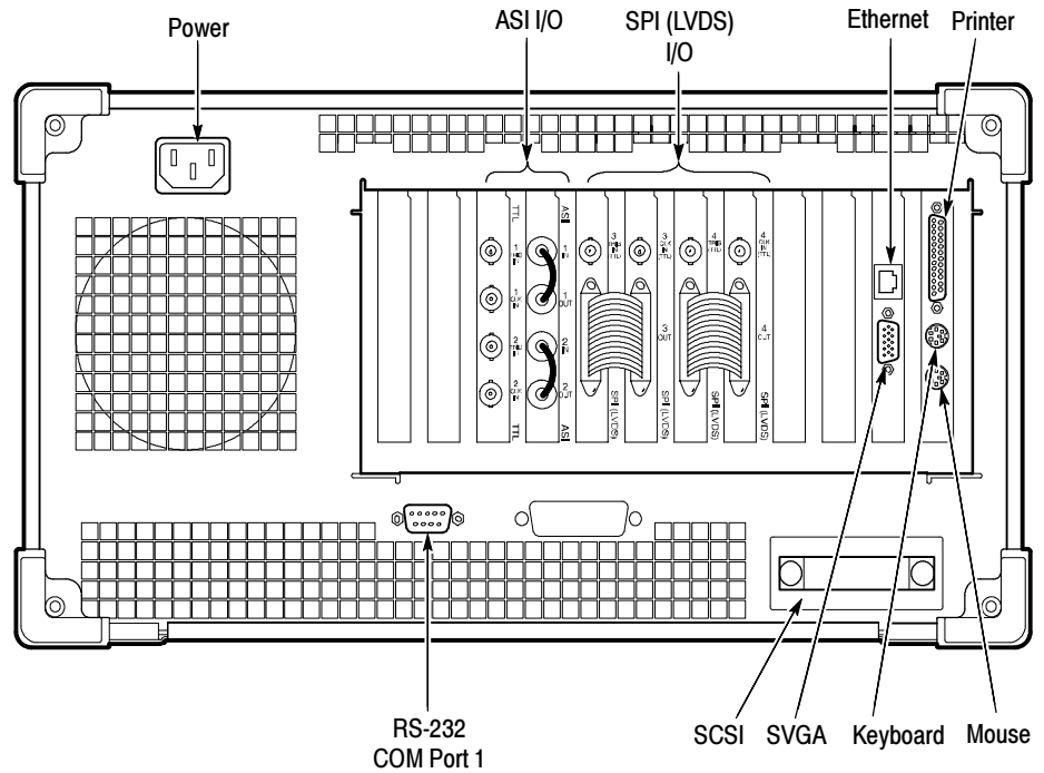
Figure 2-8: Typical initial equipment setup
