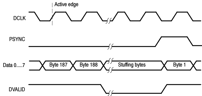
Figure 3-1: Parallel data timing, 188-byte packets
