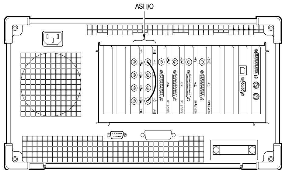
Figure 2-17: ASI cabling
